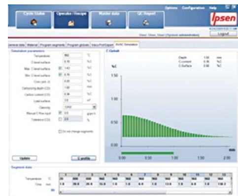
Figure 2: AvaC® Expert depicting AvaC® Simulation model.
