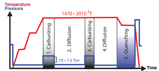
Figure 1: Typical cycle with temperature and pressure curve.
