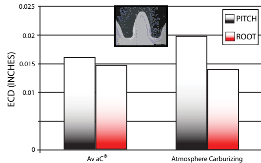
Figure 5: AvaC® vs. Other Processes: Carburizing Homogeneity
