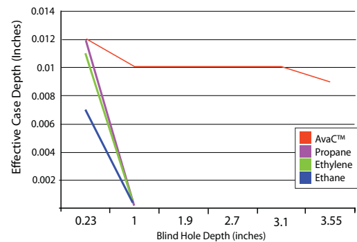
Figure 4: Surface Hardness Results
